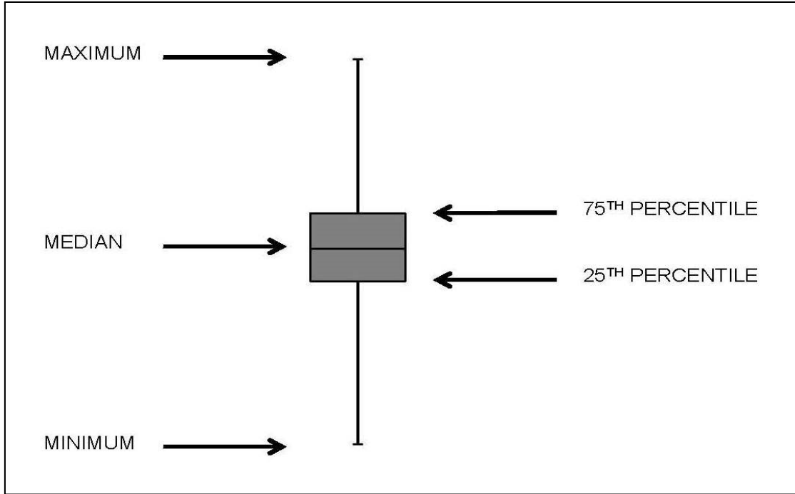
Figure 5 – Box and Whisker Plot Interpretation
